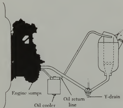
FIGURE 8-5. Oil system drain points.
